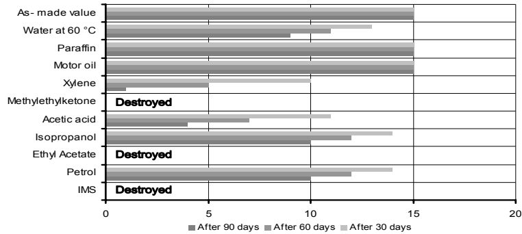
Average lap shear strengths (N/mm 2 ) vs ageing to chemical agents
